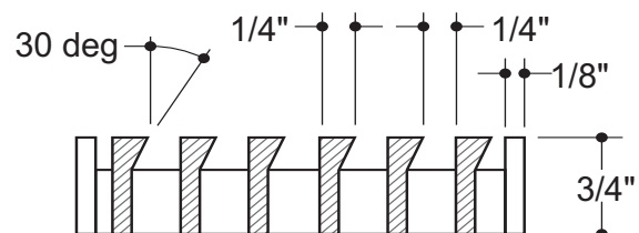
AAG 220 BAND FRAME
