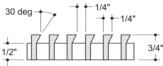
AAG 220 CORE ONLY
