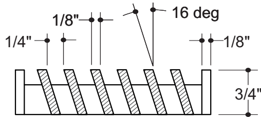
AAG 400 BAND FRAME
